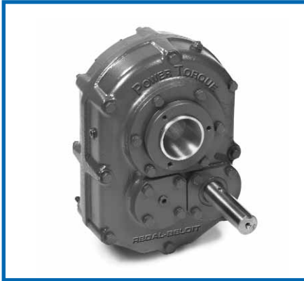
Complete Unit
