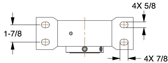
BOLT HOLE DETAILS
